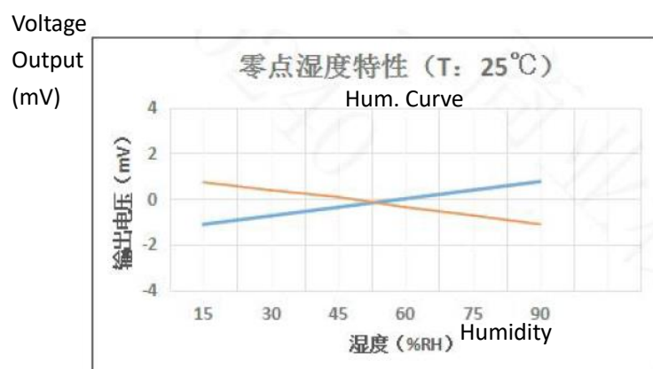
Fig7. Zero point at different humidity
