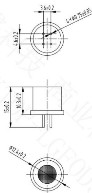
Fig1. Sensor Structure
