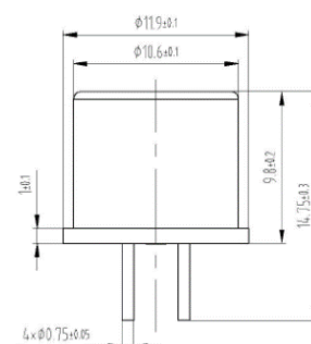
Fig1. Sensor Structure Tolerance \pm 0.1\text{mm}
