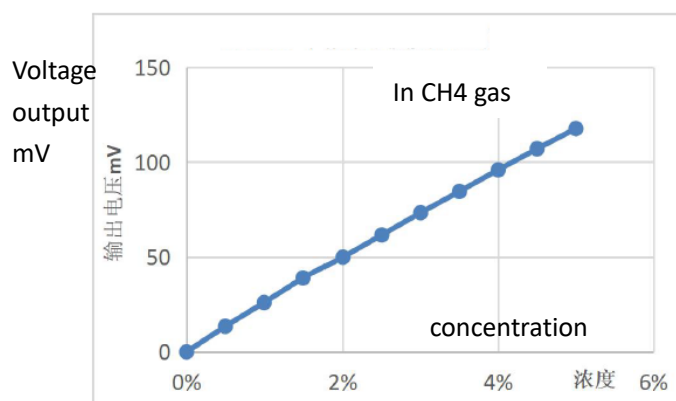
Fig3. Sensitivity Curve
