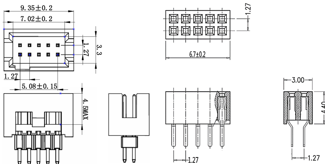
Fig2.Terminal Type (PH=2x5x1.27mm) Fig2-1Matching Terminal Description: for reference only
