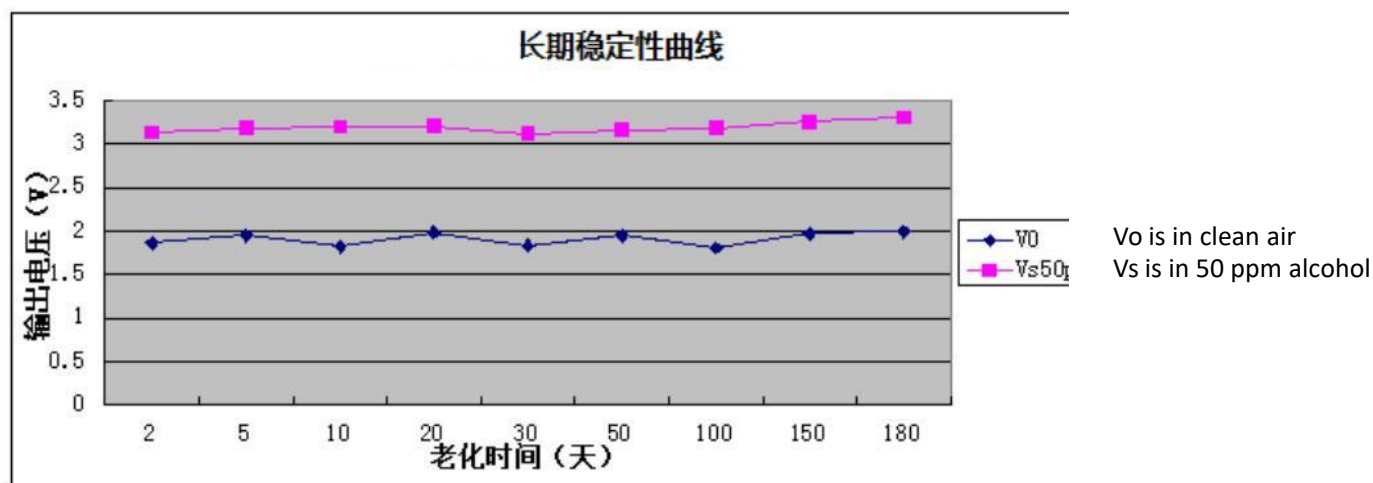
Fig7.long-term Stability
