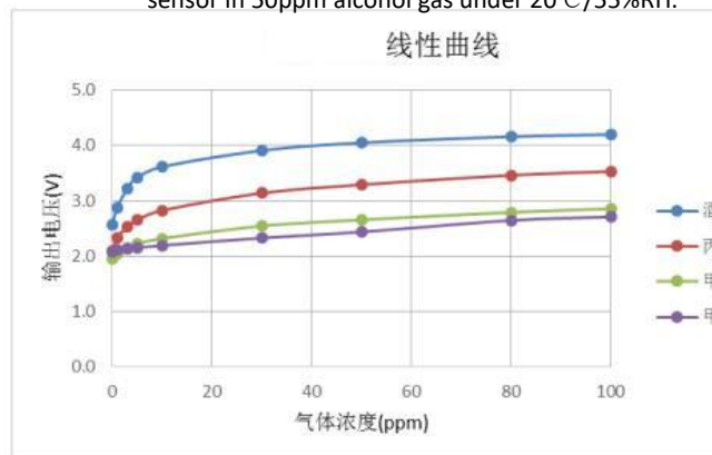
Fig6. Linearity character
