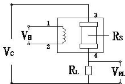
Fig2. MQ-P5 Test Circuit
