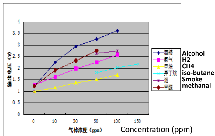
Fig6. Linearity curve
