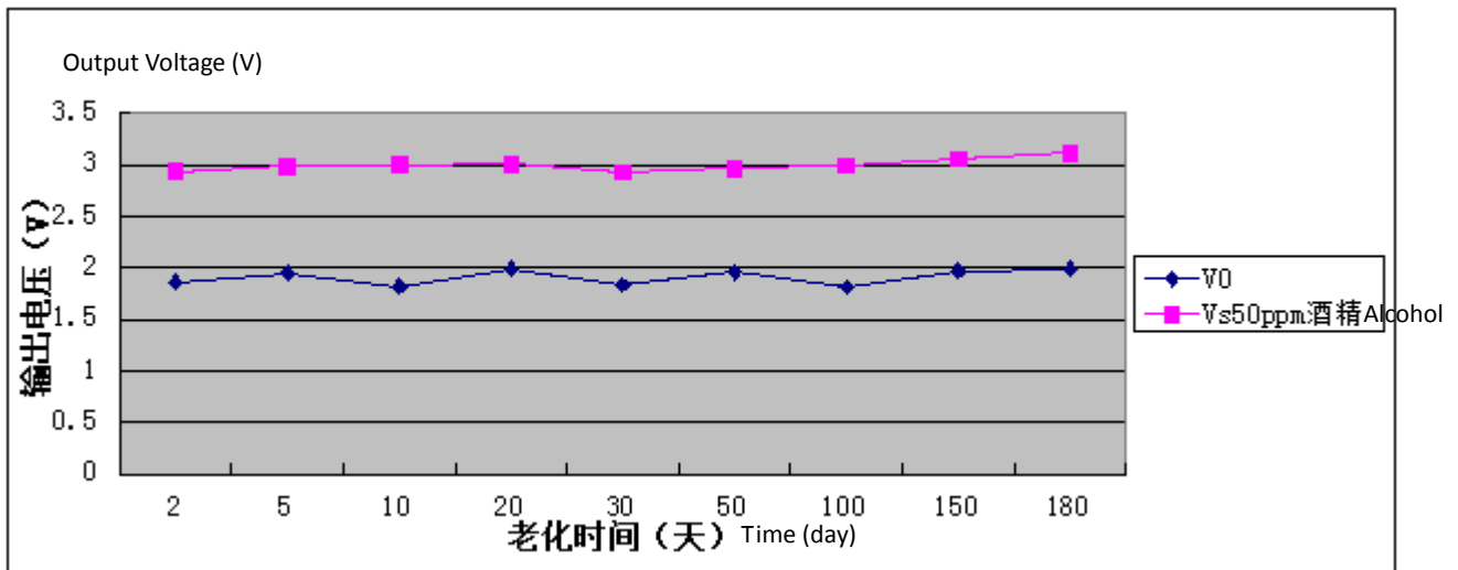
Fig7.long-term Stability of MQ-P5
