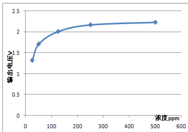
Fig5.Sensitivity Curve
