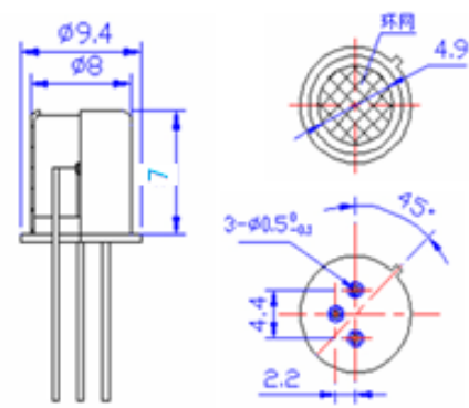
Fig1. Sensor Structure (Unit: mm)
