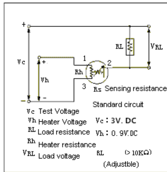
Fig2.Test Circuit
